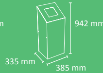
100L (upper emptying)
